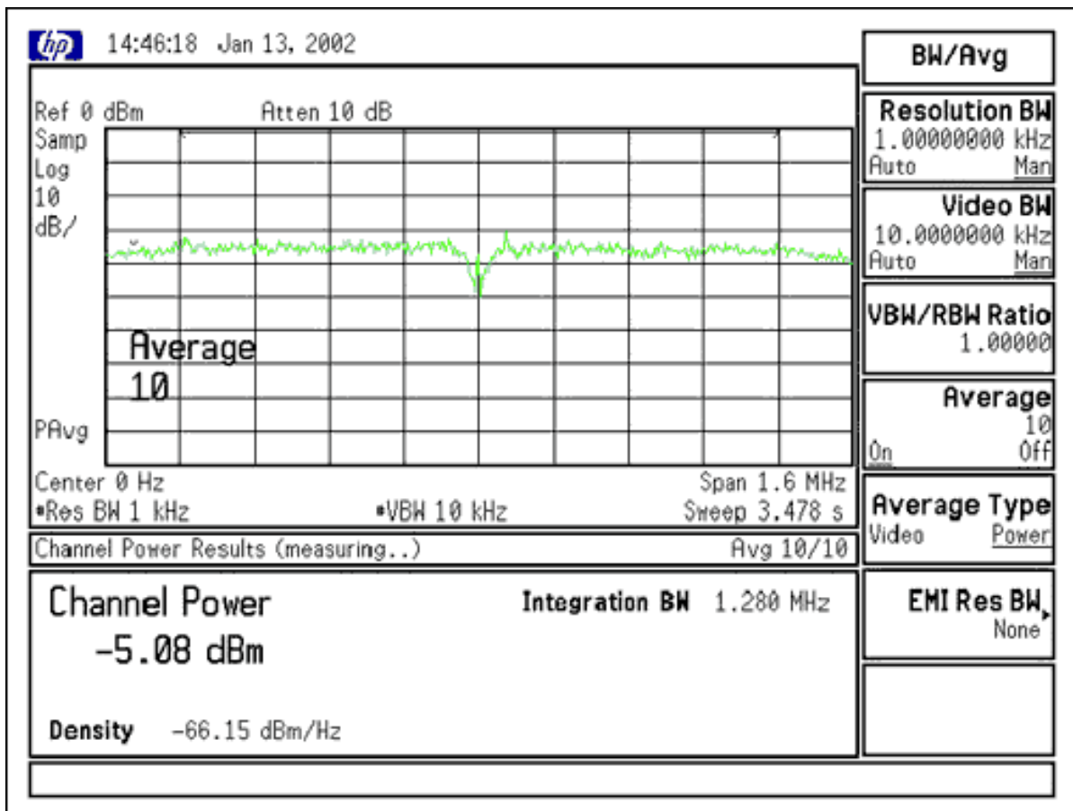
Figure 17. High-side intermodulation test
