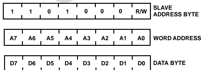
FIGURE 12. SLAVE ADDRESS, WORD ADDRESS, AND DATA BYTES
