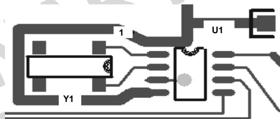
FIGURE 14. SUGGESTED LAYOUT FOR ISL12057 AND CRYSTAL
