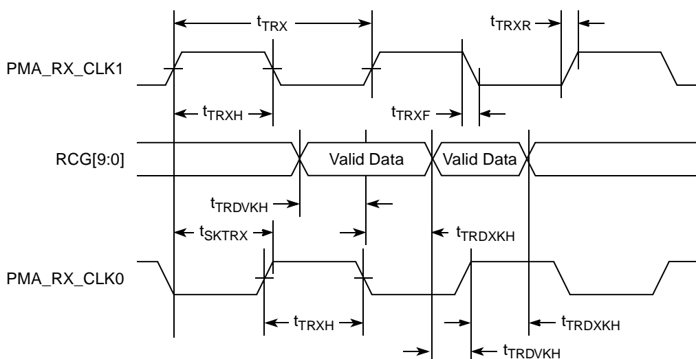
Figure 20. TBI Receive AC Timing Diagram
