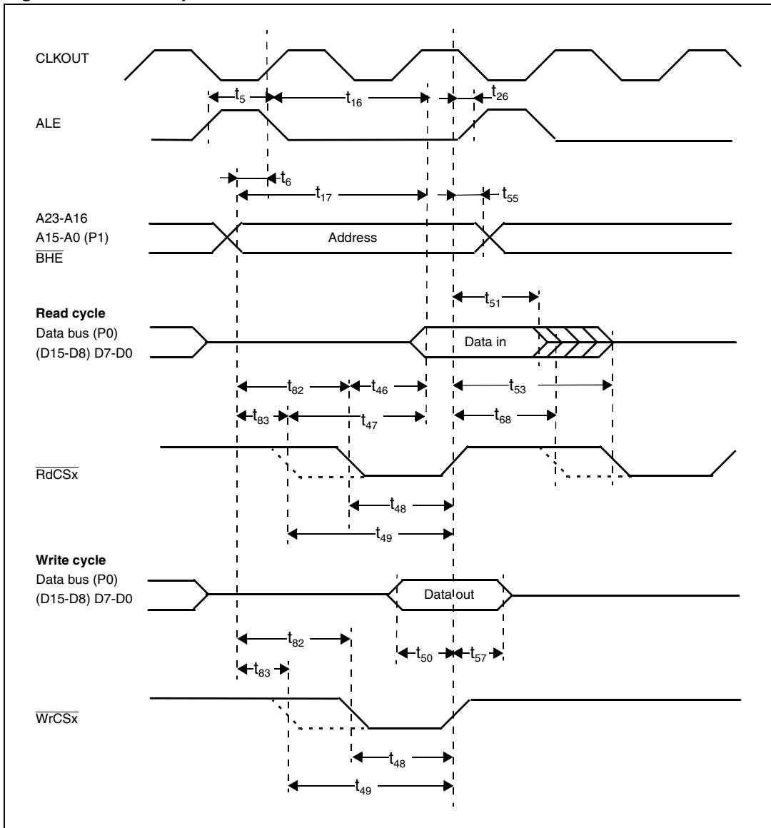
Figure 114. Demultiplexed bus with ALE and R/W \overline{CS}
