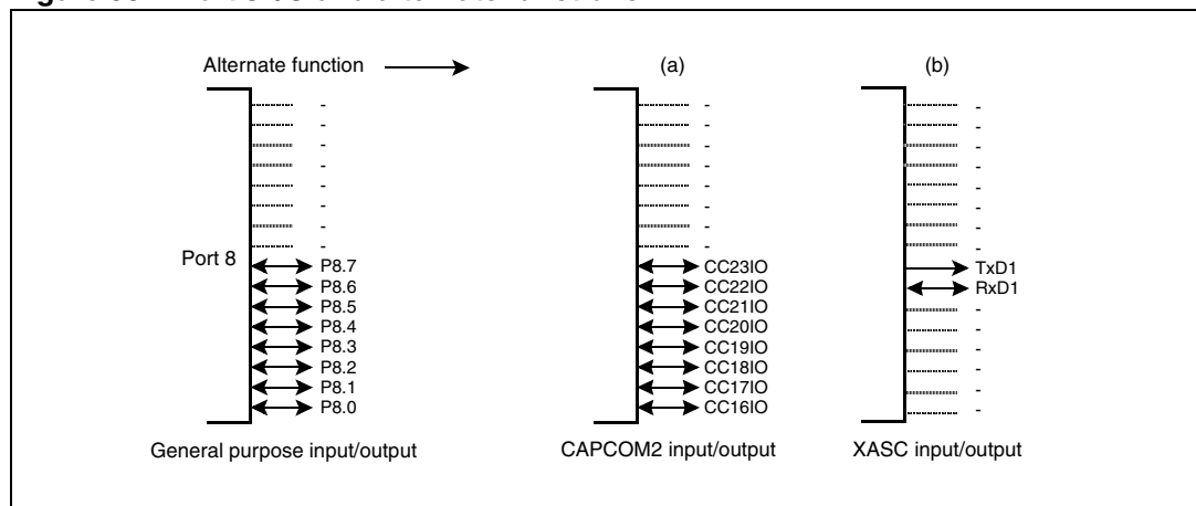
Figure 56. Port 8 I/O and alternate functions
