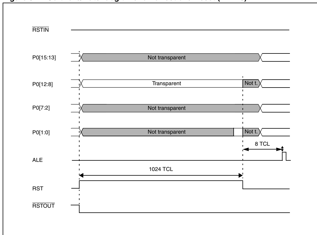
Figure 84. Software/watchdog timer unidirectional reset ( \overline{EA} = 0 )
