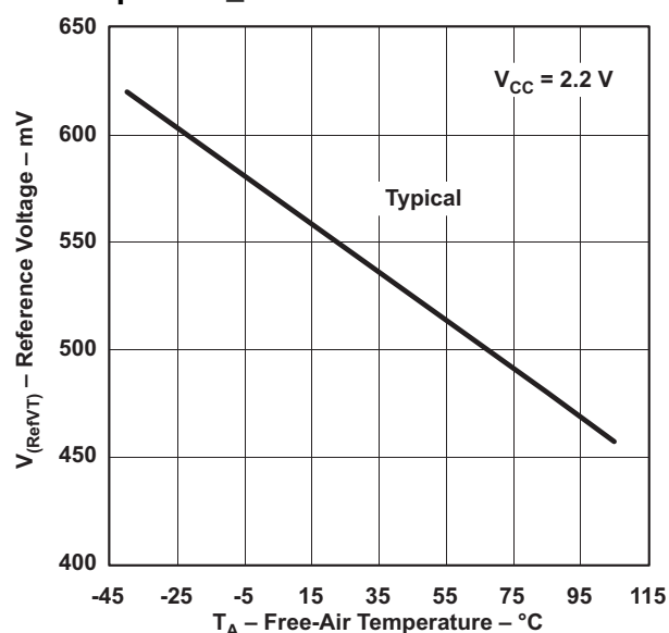
Figure 15. V_{(RefVT)} vs Temperature, V_{CC} = 2.2\text{ V}
