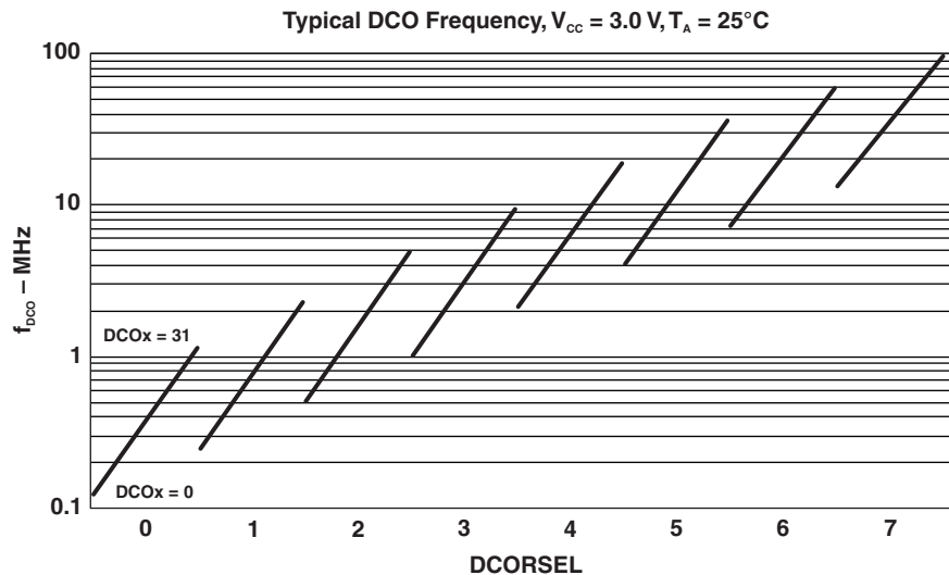
Figure 2. Typical DCO frequency
