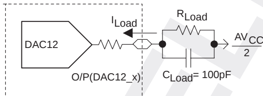
Figure 29. DAC12_x Output Resistance Tests
