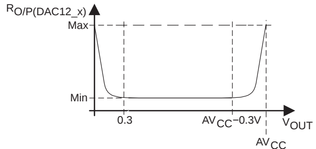
Figure 29. DAC12_x Output Resistance Tests
