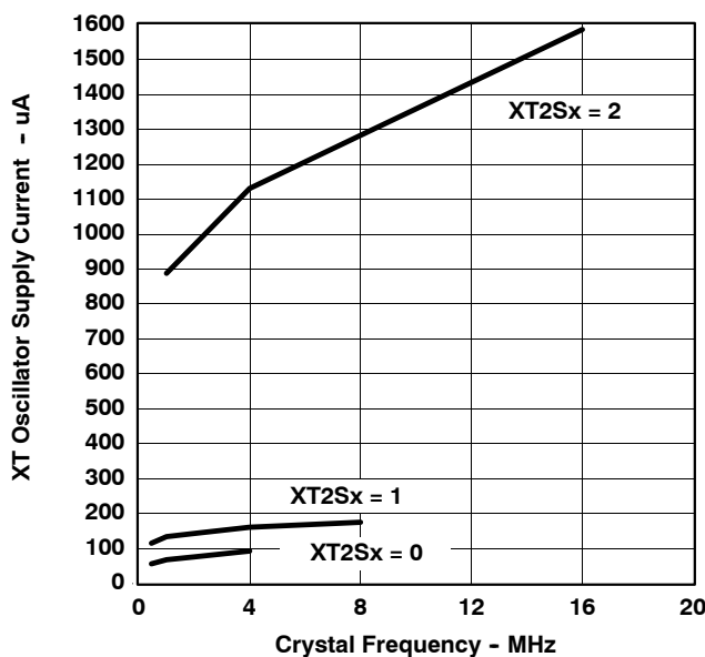
Figure 26. XT2 Oscillator Supply Current vs Crystal Frequency, C_{L,eff} = 15 pF, T_A = 25^\circ\text{C}
