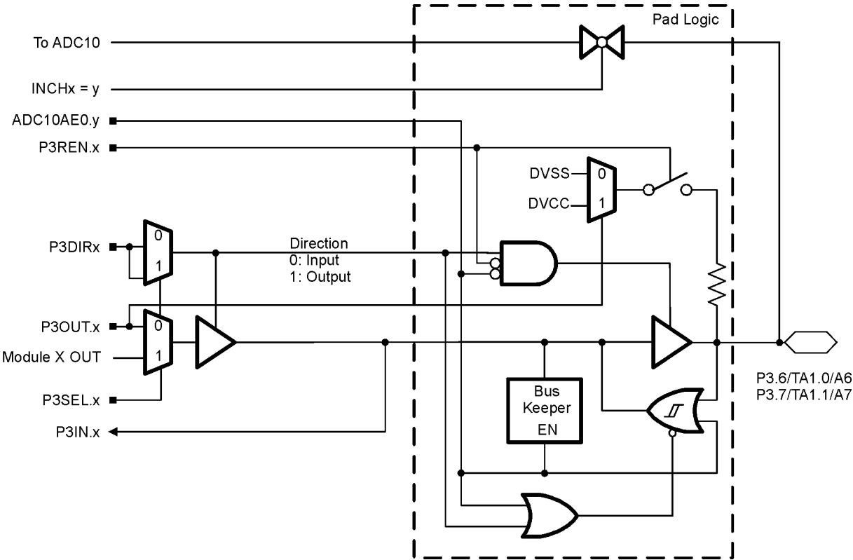
Port P3 (P3.6 and P3.7) pin functions
