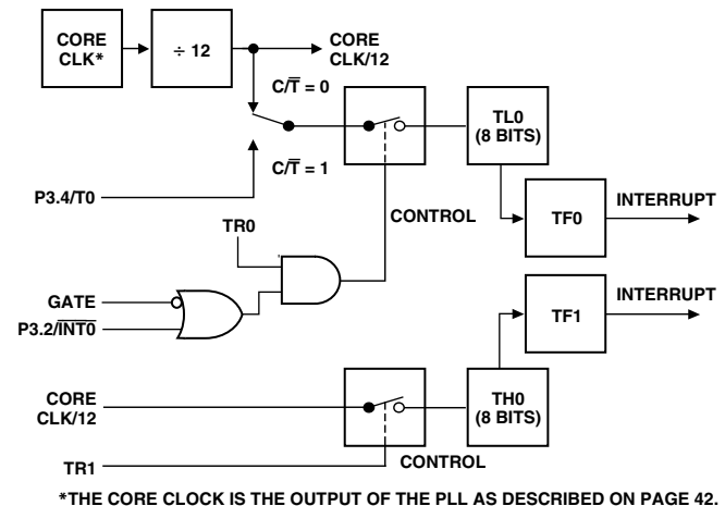
Figure 36. Timer/Counter 0, Mode 3
