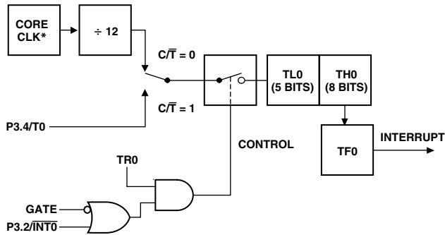
Figure 33. Timer/Counter 0, Mode 0
