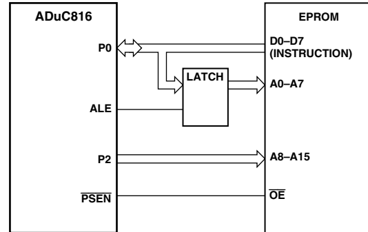
Figure 43. External Program Memory Interface
