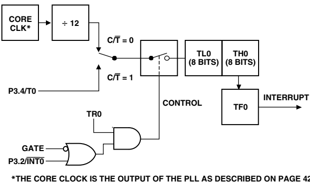
Figure 34. Timer/Counter 0, Mode 1
