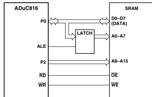
Figure 44. External Data Memory Interface (64 K Address Space)
