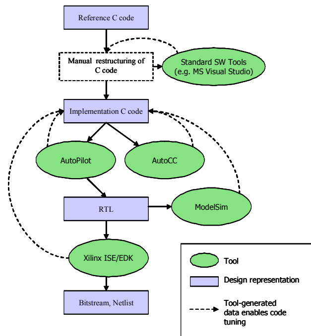
FIGURE 1. Design Flow Using the AutoPilot High-Level Synthesis Tool with Xilinx "ISE" RTL Tools
