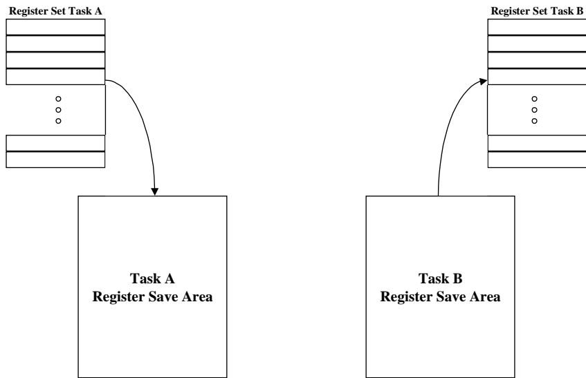
Figure 11 Context switch
